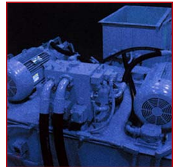
Dual motor power packs produce high displacement and provide redundant motor and pump support.
